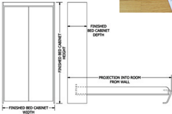
Out-to-Out dimensions of Vertical Style
