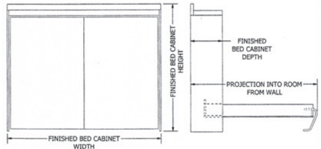
Out-to-Out dimensions of Horizontal Style
